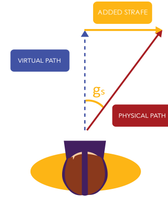
Figure 3: g_s refers to the angle to which a user is redirected, the length of the VIRTUAL PATH is defined as D_v (Eq. 1), and ADDED STRAFE is defined as D_s (Eq. 1)
